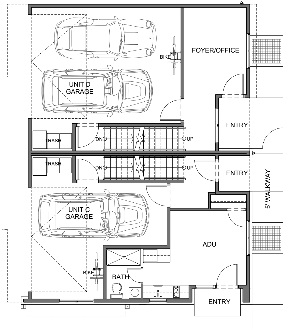
1 FIRST FLOOR PLAN OPTION 2 - BUILDING 2 SCALE: 1/8" = 1'-0"
