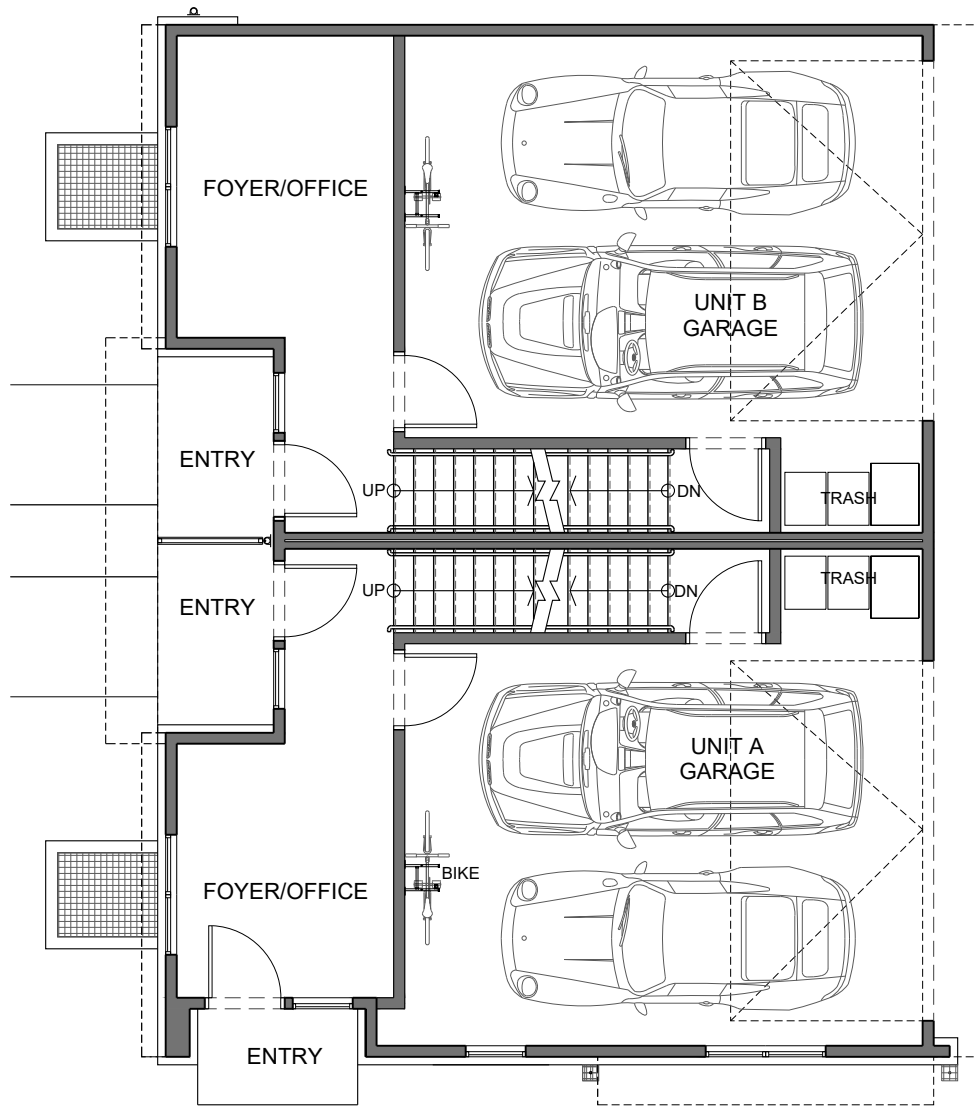
1 FIRST FLOOR PLAN OPTION 2 - BUILDING 1 SCALE: 1/8" = 1'-0"
